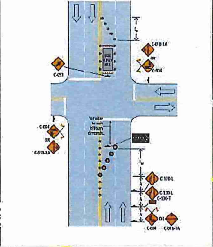
Figure 11.1: Left Lane Closure (For BSA) – Multi-Lane Intersections – Short and Long Duration
