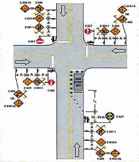
Figure 11.2: Intersection Lane Closure – Two-Lane, Two-Way Roadway with TCPs (Near Side) – Short and Long Duration
